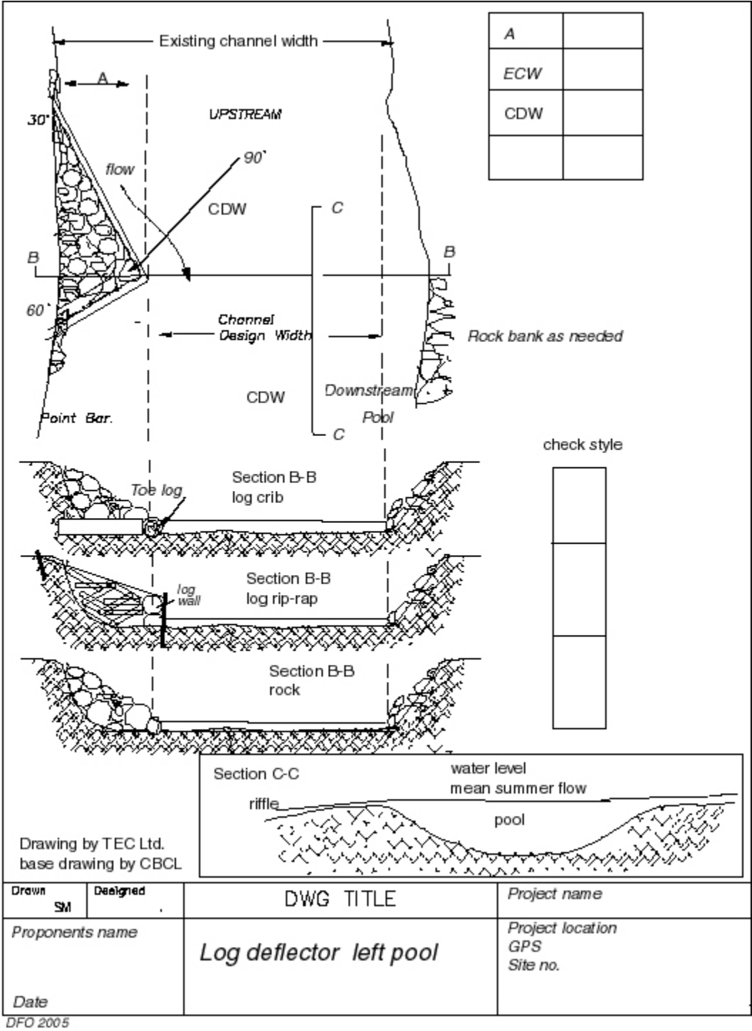
Figure 2 Deflector
